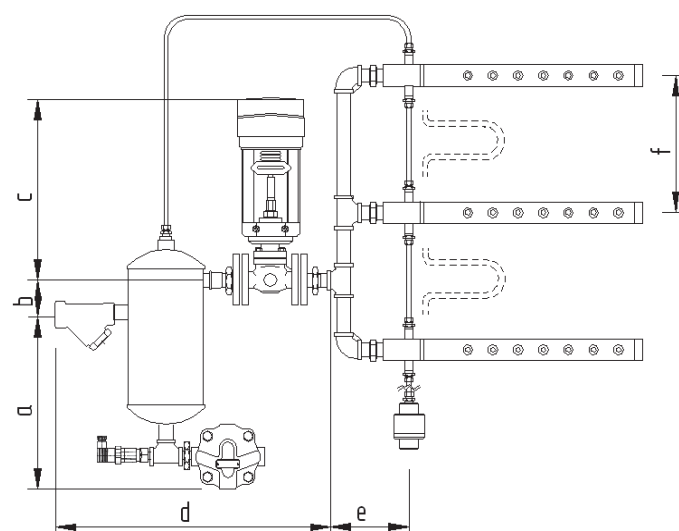
*Steam Injection system Type C (Mixed materials)
